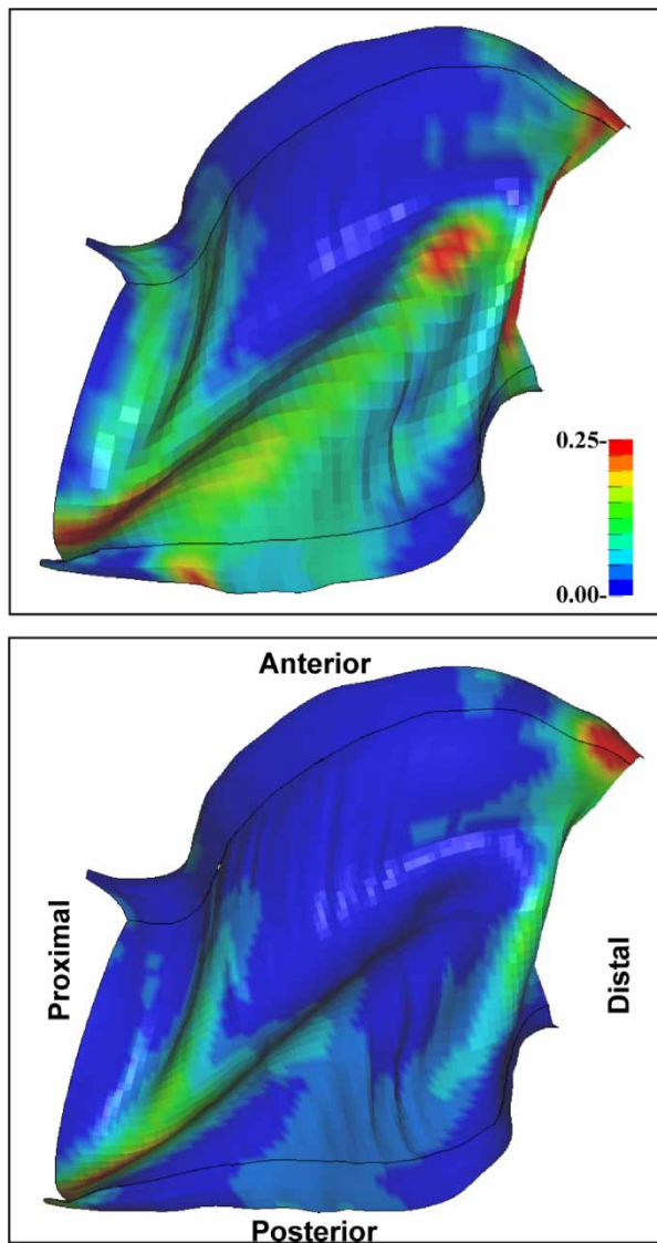
Figure 5. Top panel—fringe plot of 1st principal Green-Lagrange strains for a coarse mesh of the inferior glenohumeral ligament complex (1650 shell elements). Model deformation is correct, but mesh induced “hot-spots” are prevalent. Bottom panel—refined mesh of the inferior glenohumeral ligament complex (6600 shell elements) showing considerable differences in strains when compared to the coarse mesh, especially in areas of ligament buckling. Average strains from this final mesh were less than one percent different than a mesh with twice as many elements. Reprinted from Ellis et al. (2006a) with permission.
